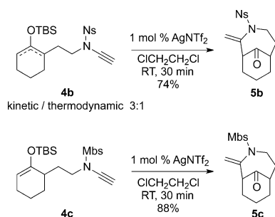
Scheme 2. Variation of the electron-withdrawing group. Mbs = p -methoxybenzenesulfonyl, Ns = 2-nitrobenzenesulfonyl.
