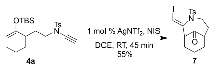
Scheme 4. Trapping alkenylsilver intermediates. DCE = 1,2-dichloroethane, NIS = N -iodosuccinimide.
