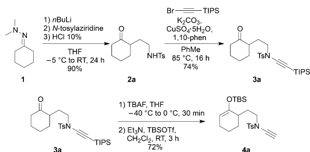
Scheme 1. Synthesis of the silyl enol ether 4a . TBAF = tetra- n -butylammonium fluoride, TBS = tert -butyldimethylsilyl, Tf = trifluoromethanesulfonyl, THF = tetrahydrofuran, TIPS = triisopropylsilyl, Ts = 4-toluenesulfonyl.
