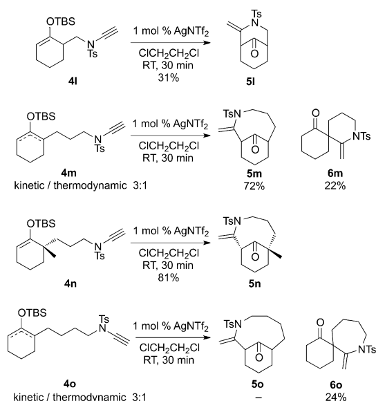
Scheme 3. Modification of the spacer length.
