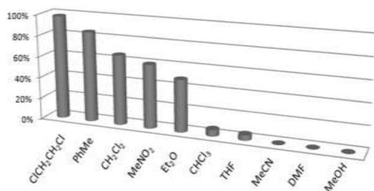
Figure 1. Screenings of solvents.
